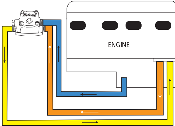
Wet Sump System Internal Pump
