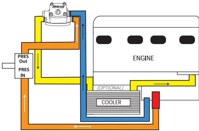
Wet Sump System External Pump
