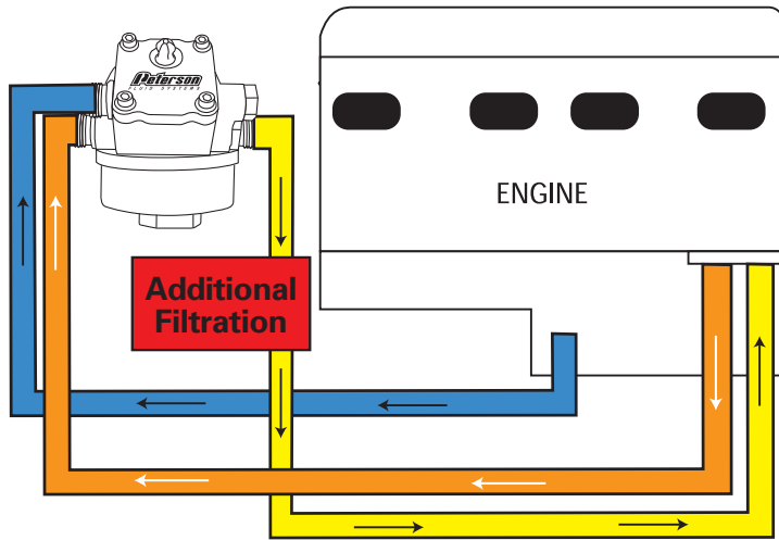
Wet Sump System Internal Pump
