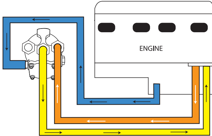
Wet Sump System Internal Pump
