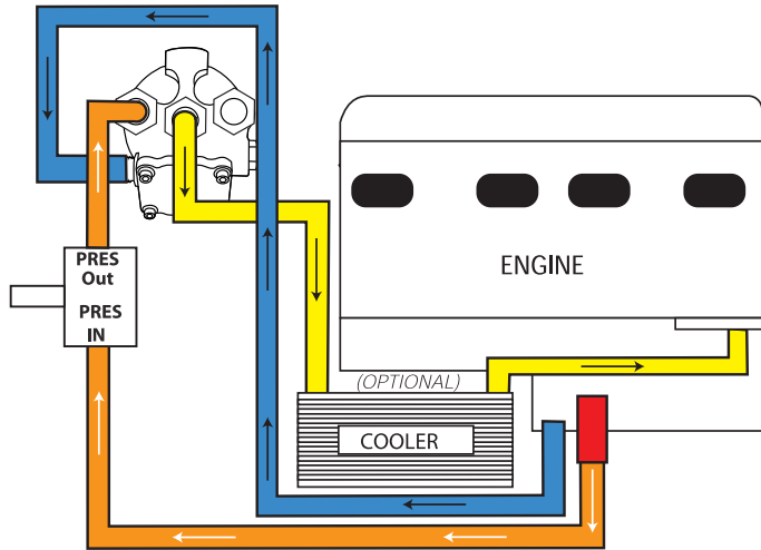
Wet Sump System External Pump
