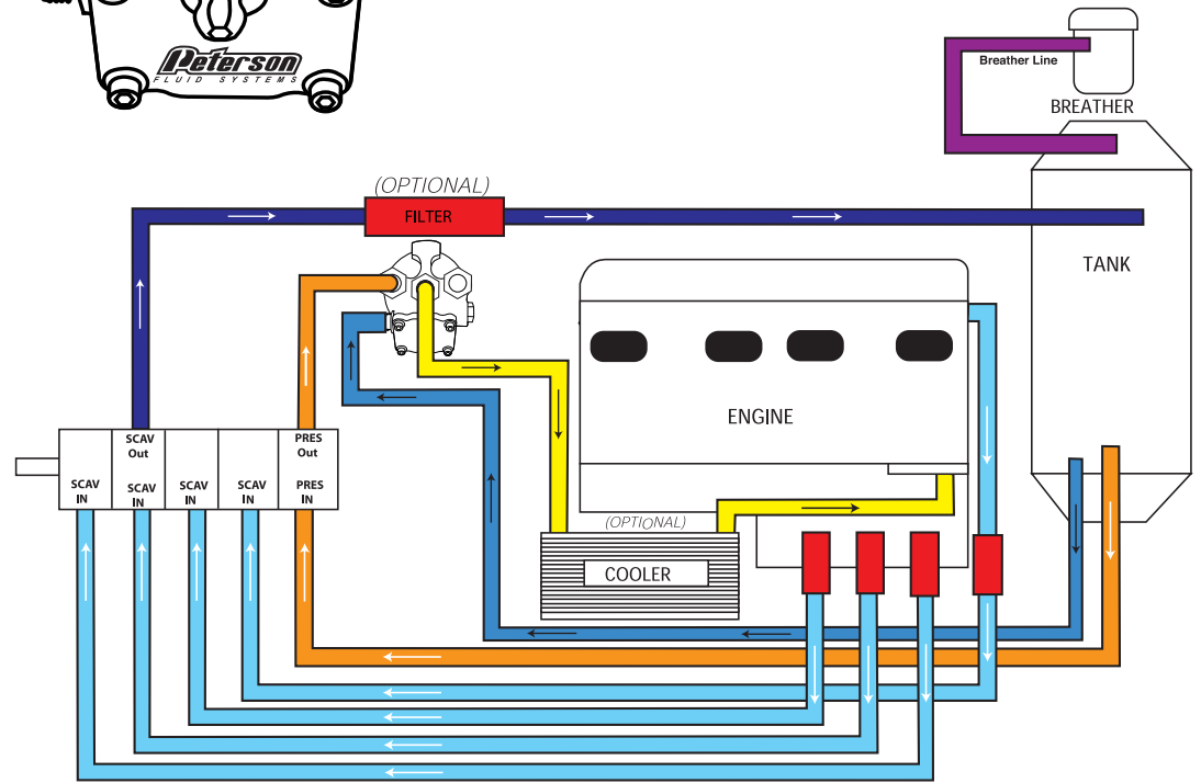
Dry Sump System
